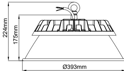
Universal Reflector
