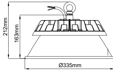
Universal Reflector
